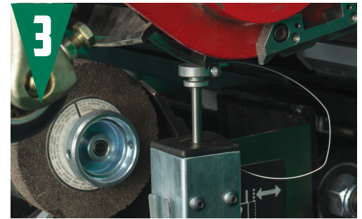
ACCU-POSITIONING GAUGE
